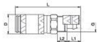
Hose connector
