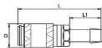
Hose stem
